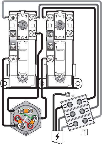
Electrical connection, diagram - 300-1000 l.
